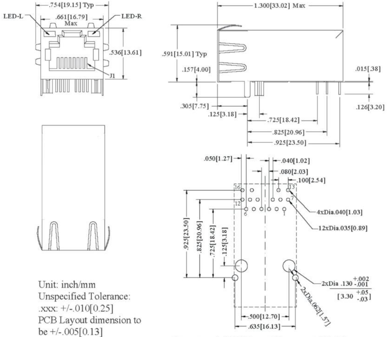
Recommended PCB Layout Component Side View
