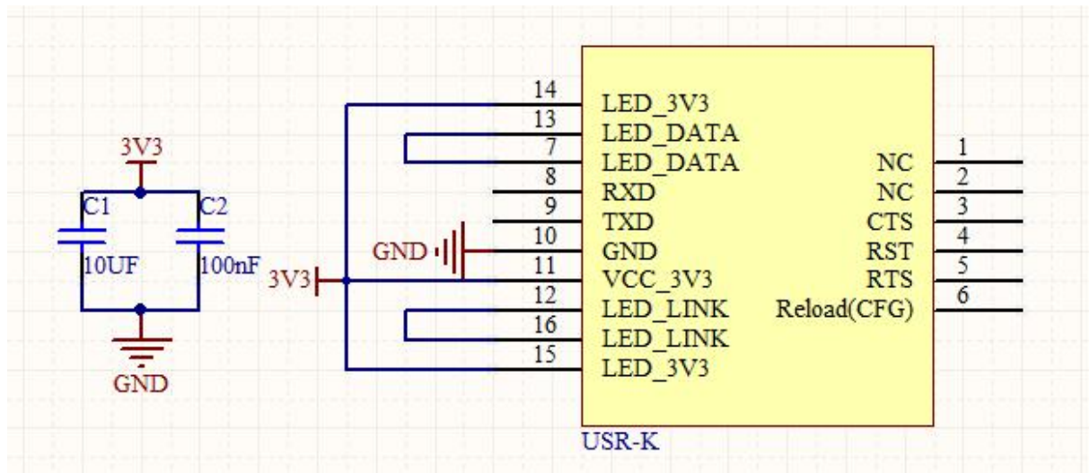
Diagram 4-5 connection diagram
