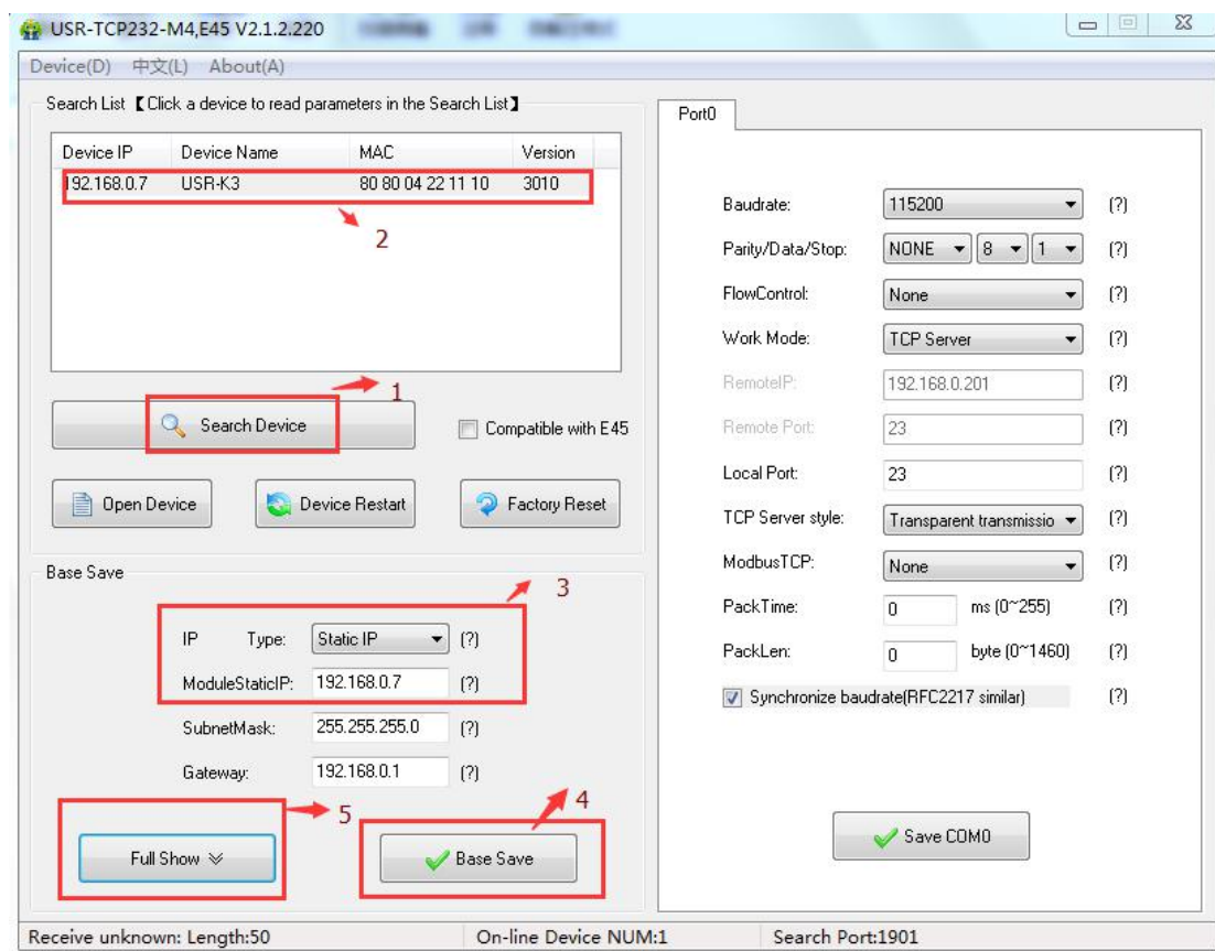
Diagram 5-1 Setup software
